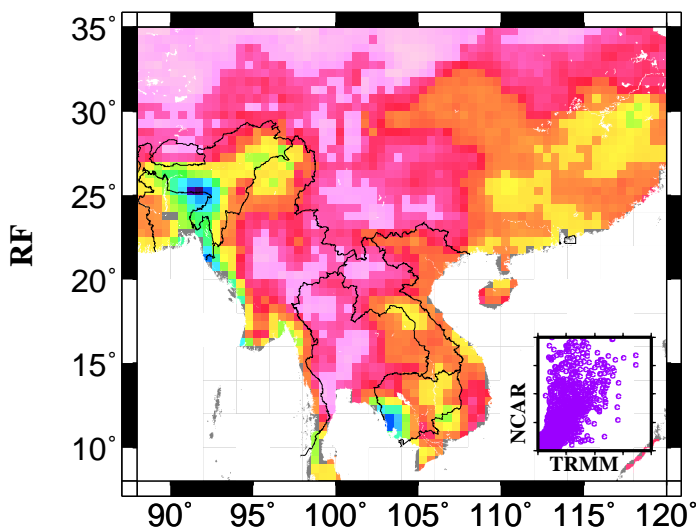
SEA Average PPTN, ET & RF Map – 1998–2006
